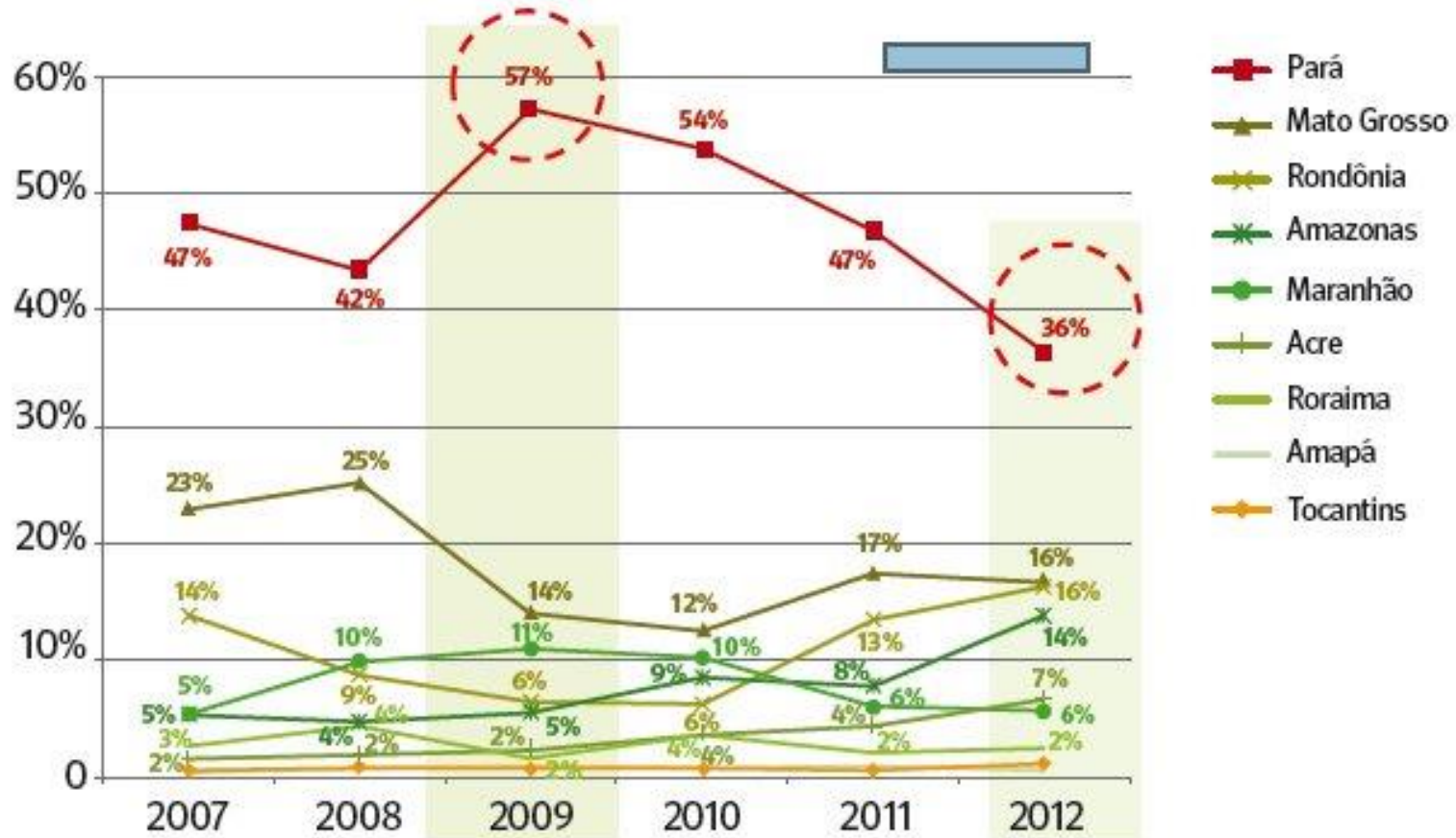
Graph 2. Participation by the states in deforestation per year (period of 2007 to 2012)
